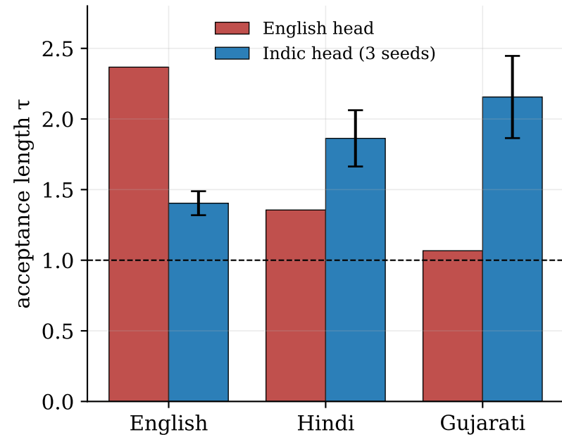
(a) FLORES (in-domain)
