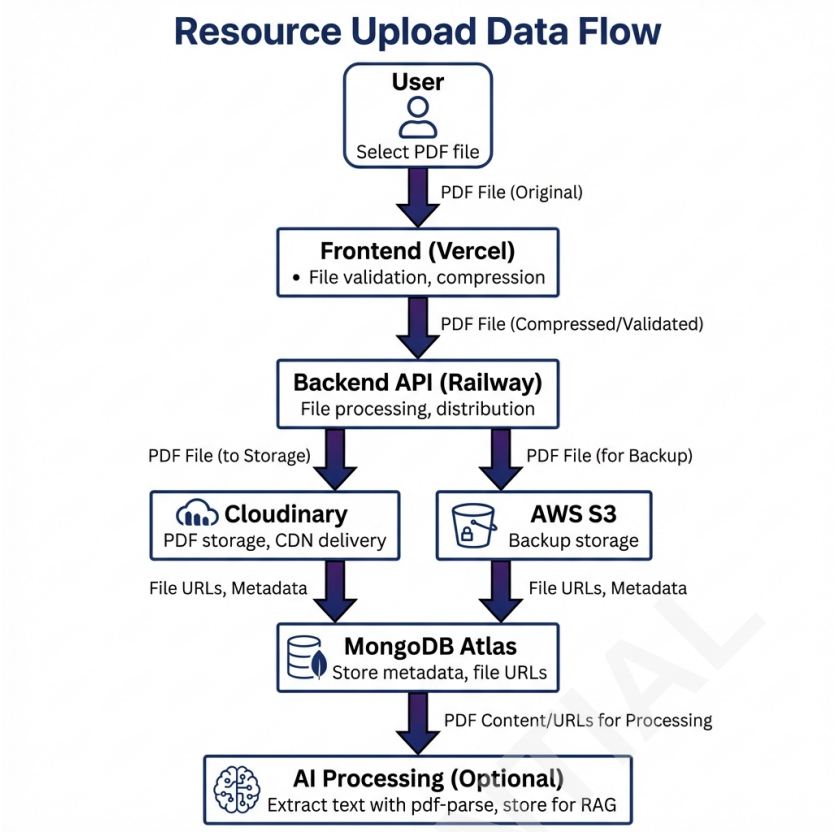
Figure: Resource Upload Data Flow
