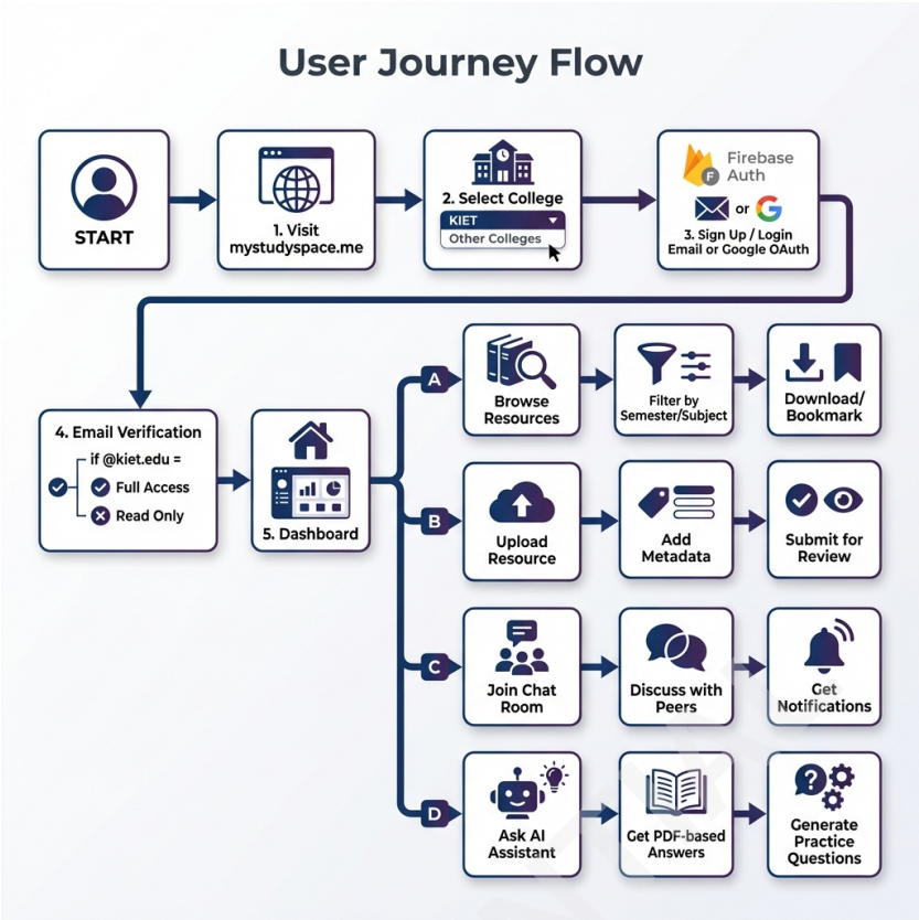
Figure: User Journey Flow
