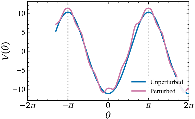
Effect of sine perturbation on V(\theta)
