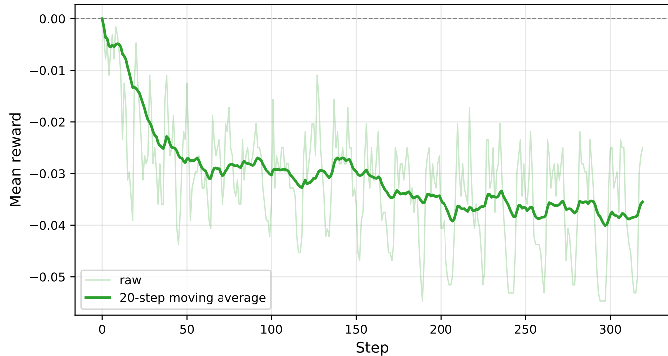
Mean Reward - 4x4/output
