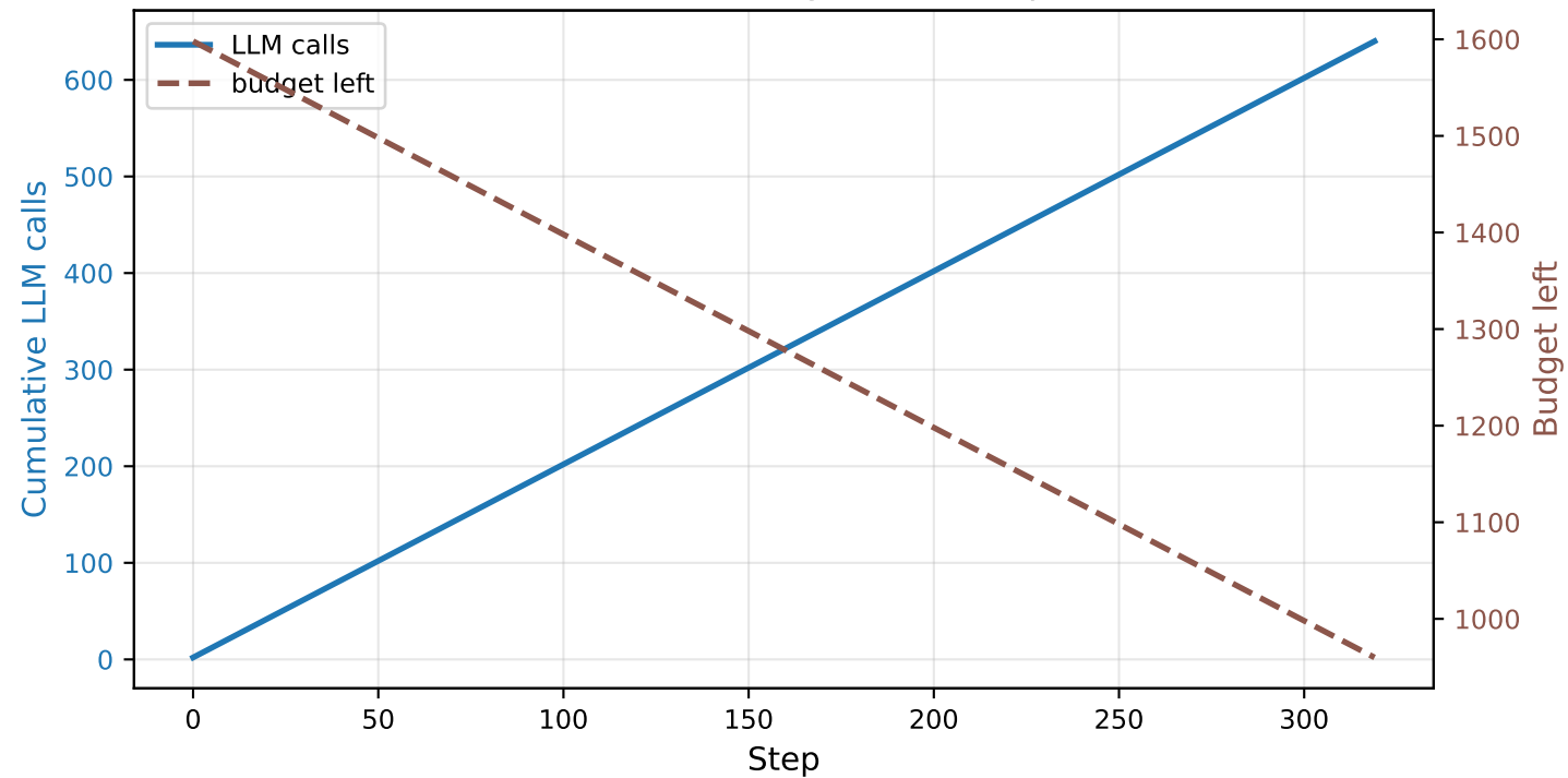
LLM Calls and Budget - 4x4/output
