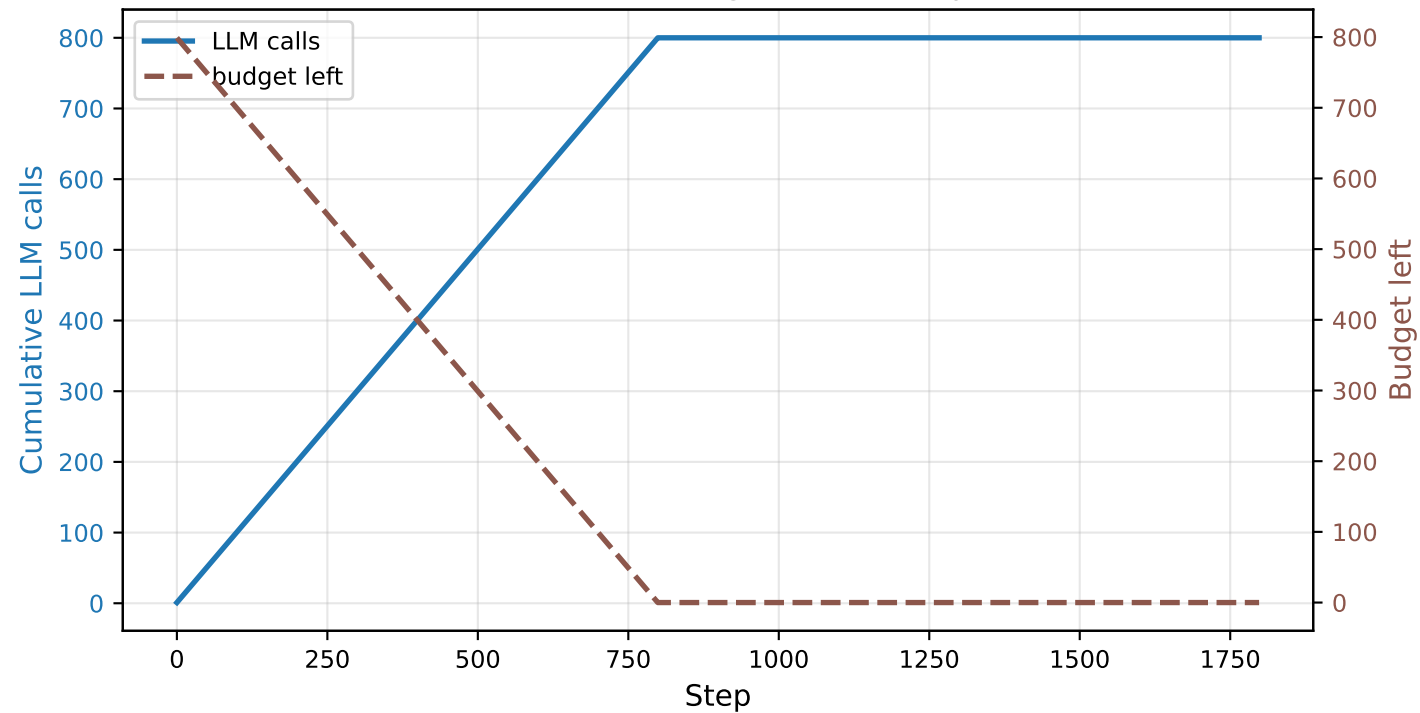
LLM Calls and Budget - 7x28/output
