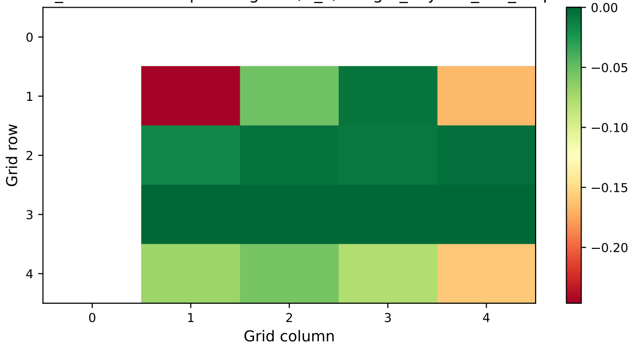
mean_reward Heatmap - Hangzhou/4_4/safegat_cityflow_live_output
