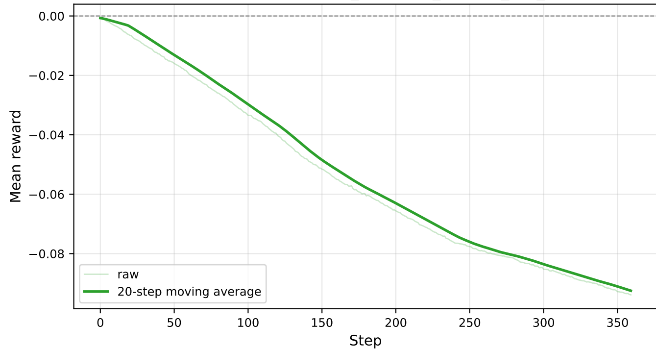
Mean Reward - Hangzhou/4_4/safegat_cityflow_live_output
