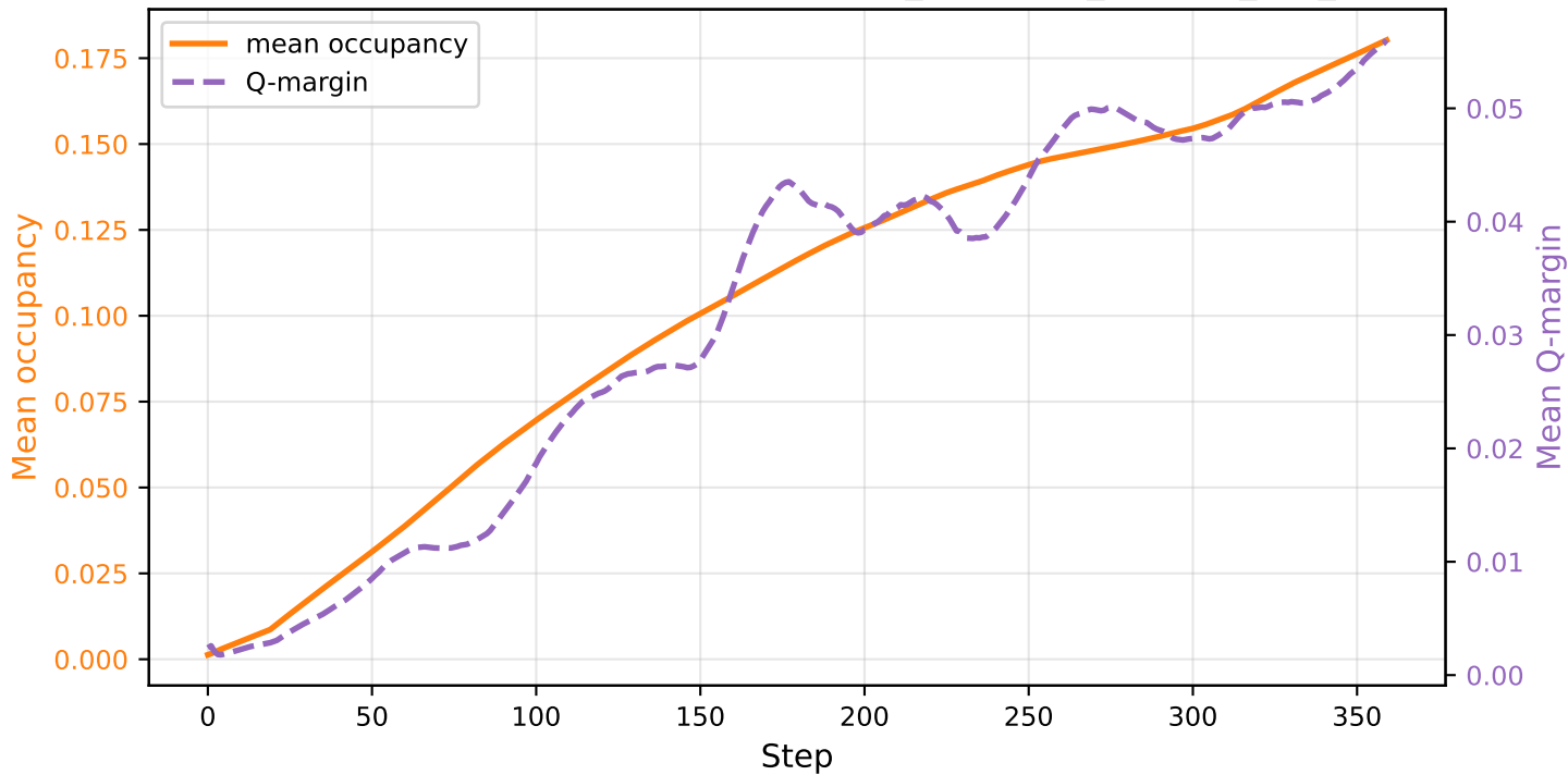
Occupancy and Confidence Margin - Jinan/3_4/safegat_cityflow_live_output
