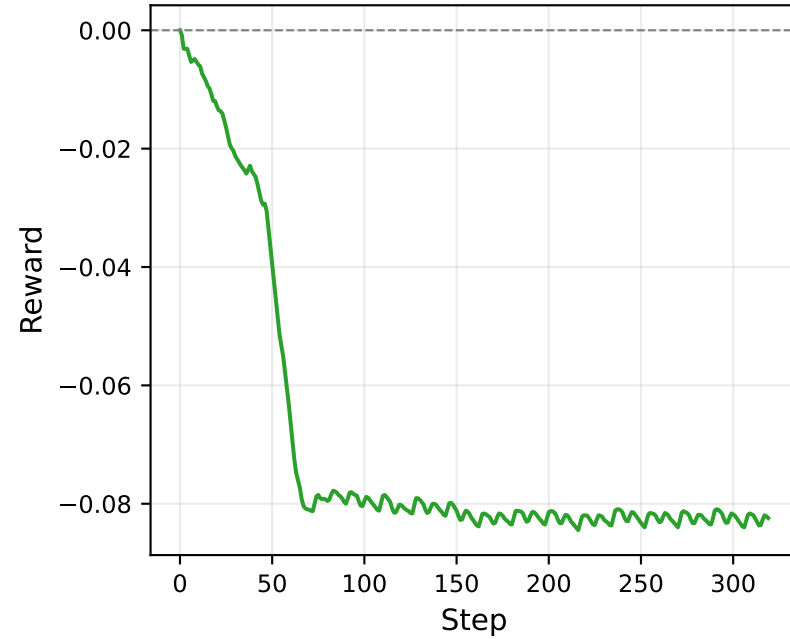
Mean reward
