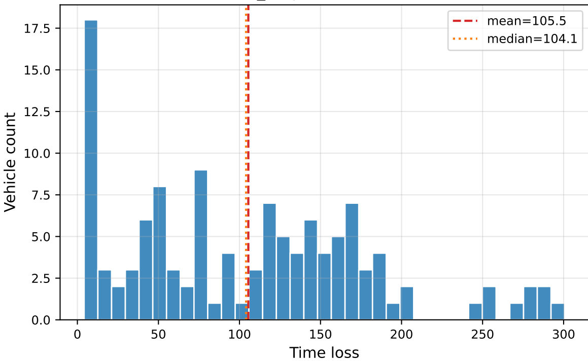
Time loss Distribution - LLM_outputs/4x4/llama-3.3-70b-versatile/output
