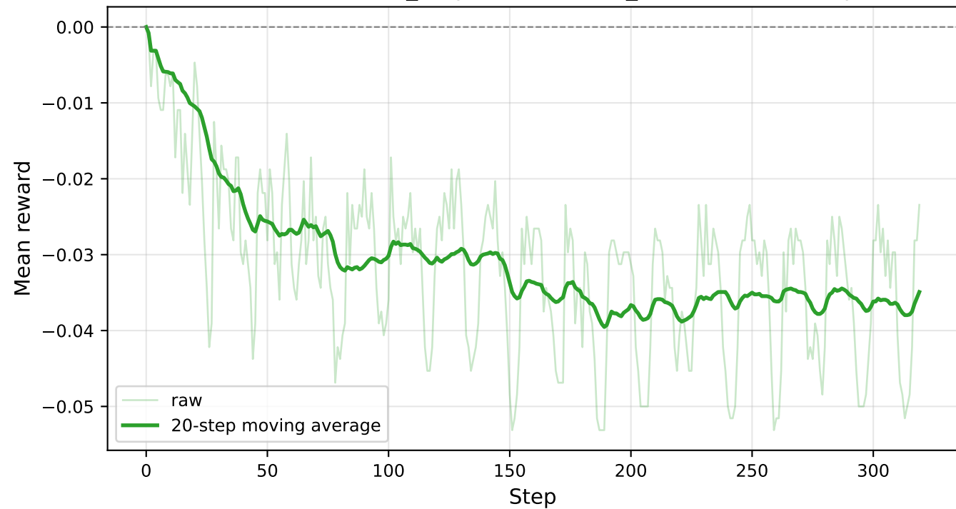
Mean Reward - LLM_outputs/4x4/llama_3.1-8b-instant/output
