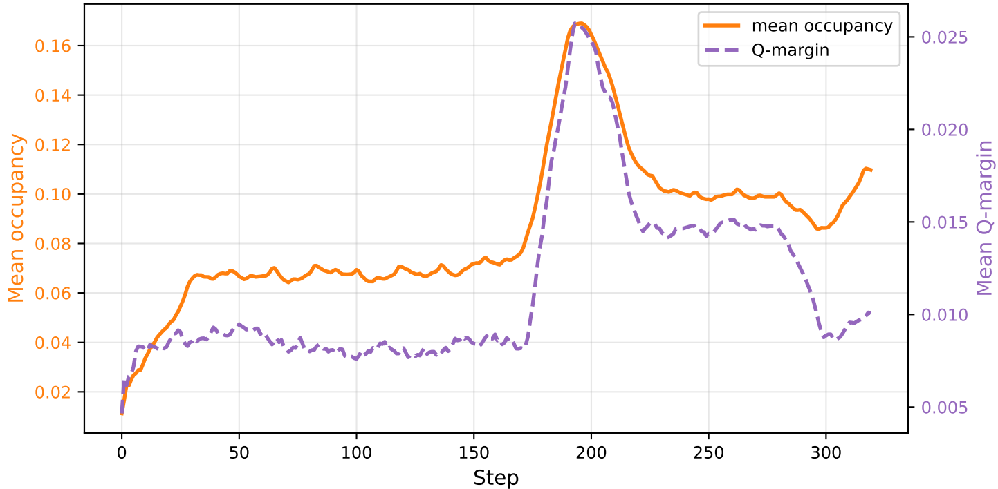
Occupancy and Confidence Margin - LLM_outputs/4x4/meta-llamallama-4-scout-17b-16e-instruct/output
