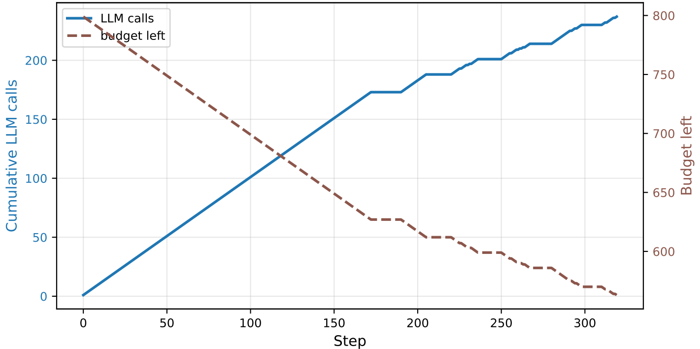
LLM Calls and Budget - LLM_outputs/4x4/meta-llamallama-4-scout-17b-16e-instruct/output
