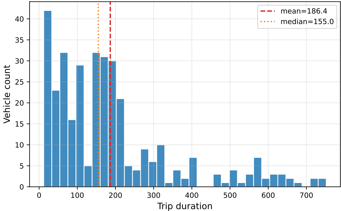
Trip duration Distribution - LLM_outputs/4x4/meta-llamallama-4-scout-17b-16e-instruct/output
