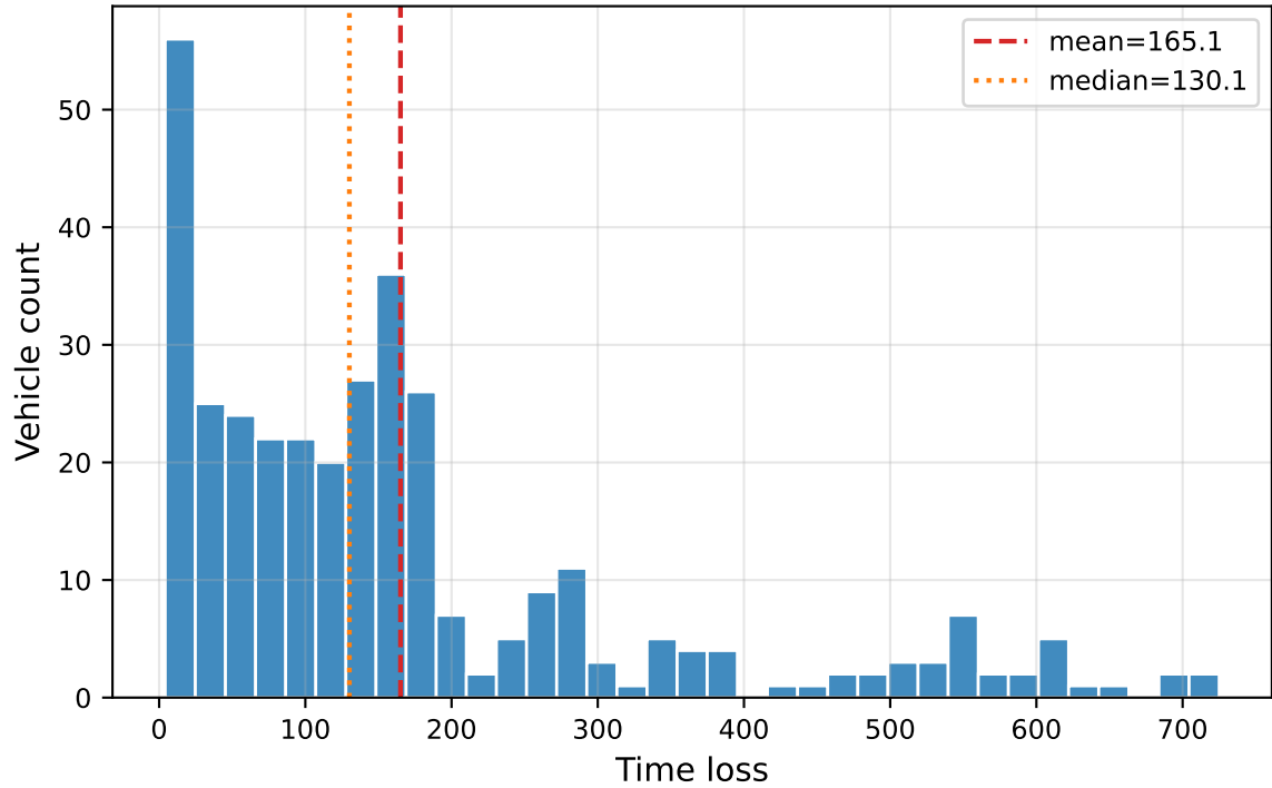
Time loss Distribution - LLM_outputs/4x4/meta-llamallama-4-scout-17b-16e-instruct/output
