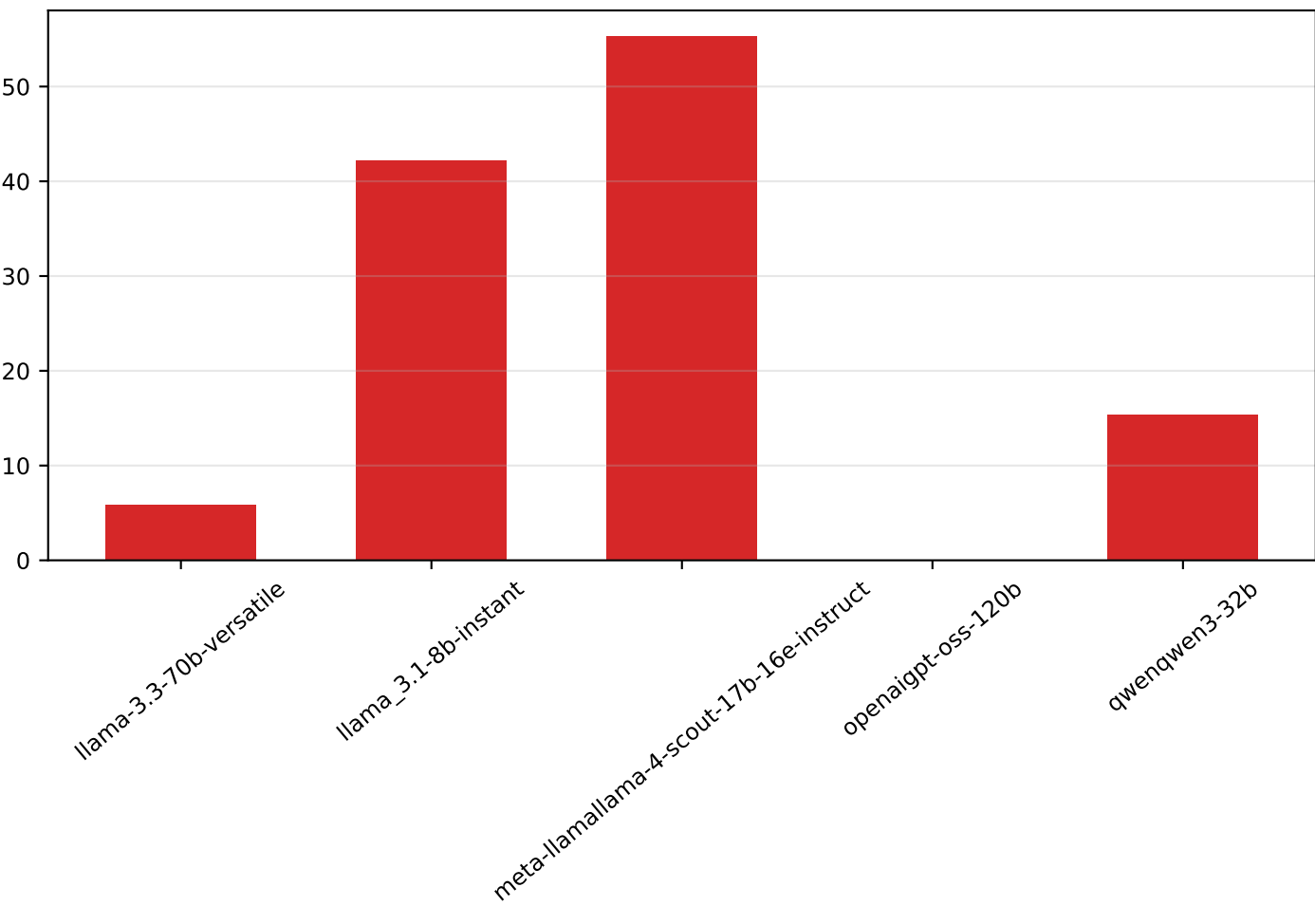
Override rate (%)
