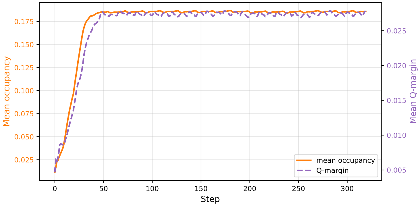
Occupancy and Confidence Margin - LLM_outputs/4x4/openaigpt-oss-120b/output
