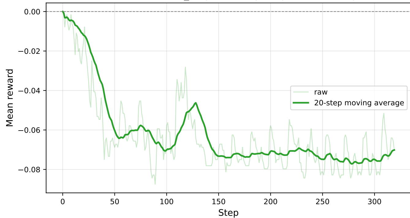
Mean Reward - LLM_outputs/4x4/qwenqwen3-32b/output
