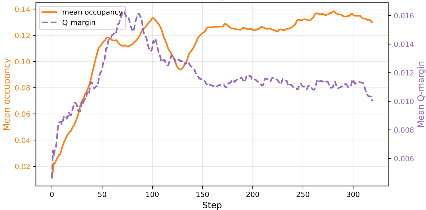
Occupancy and Confidence Margin - LLM_outputs/4x4/qwenqwen3-32b/output
