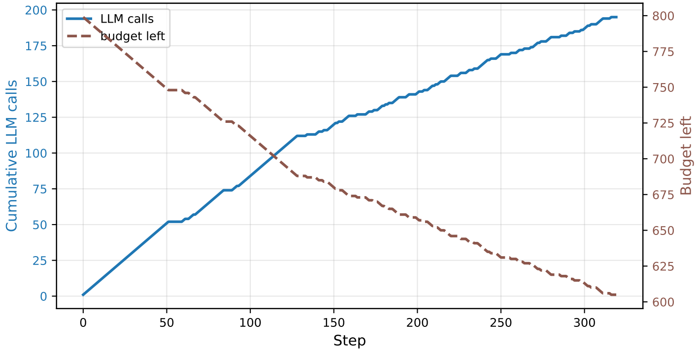
LLM Calls and Budget - LLM_outputs/4x4/qwenqwen3-32b/output
