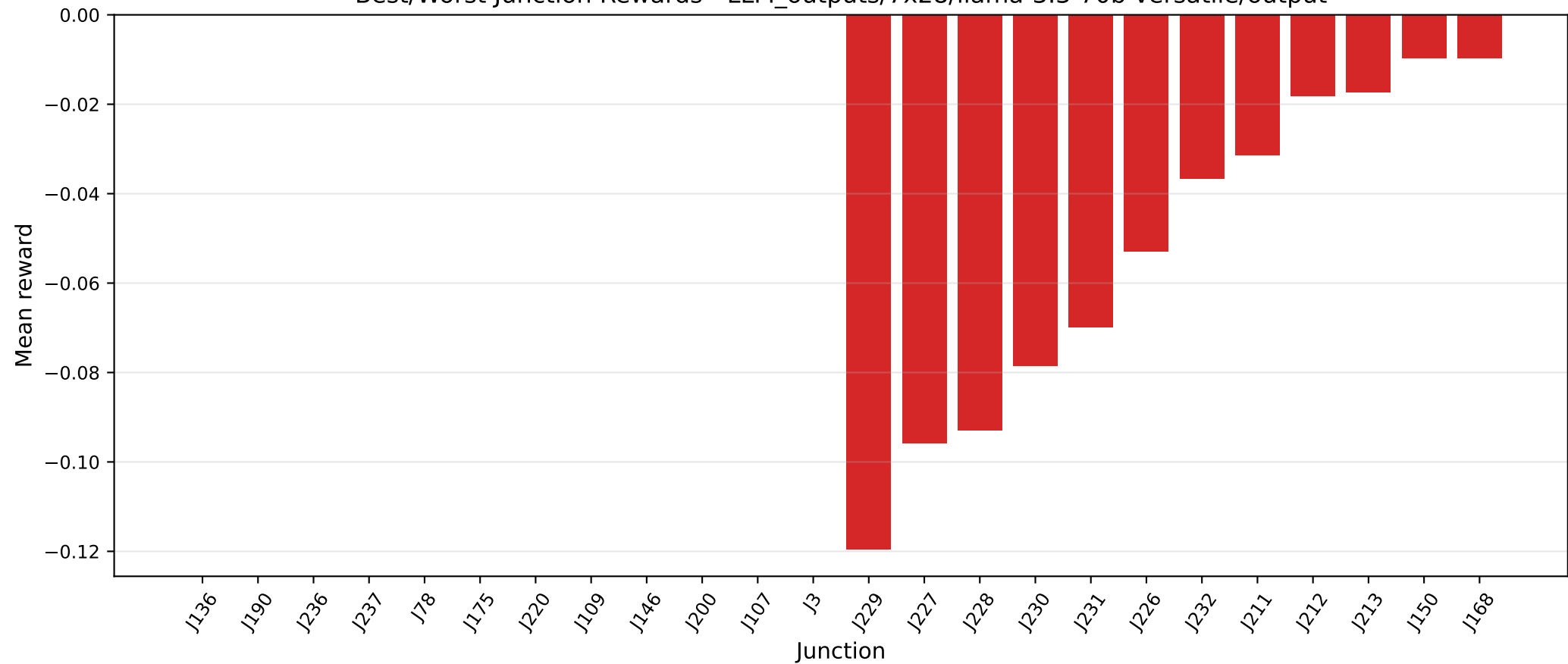
Best/Worst Junction Rewards - LLM_outputs/7x28/llama-3.3-70b-versatile/output
