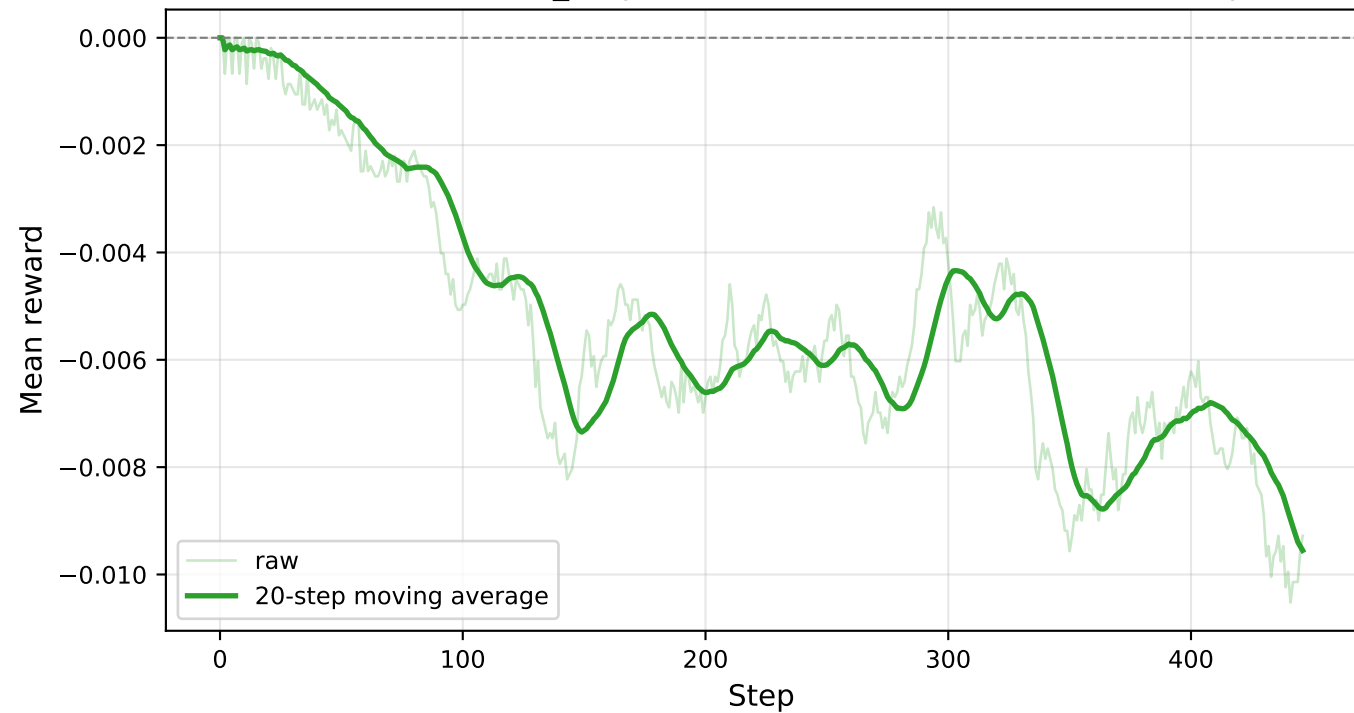
Mean Reward - LLM_outputs/7x28/llama-3.3-70b-versatile/output
