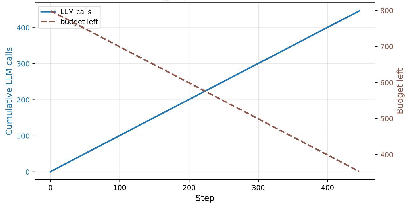
LLM Calls and Budget - LLM_outputs/7x28/llama-3.3-70b-versatile/output
