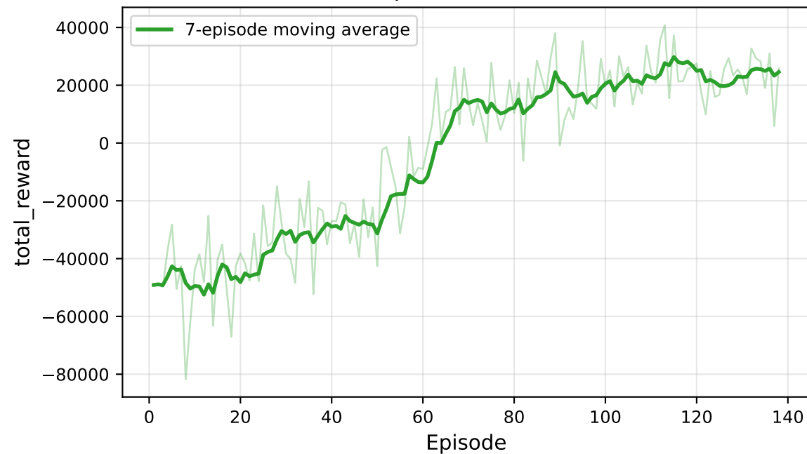
Episode reward
