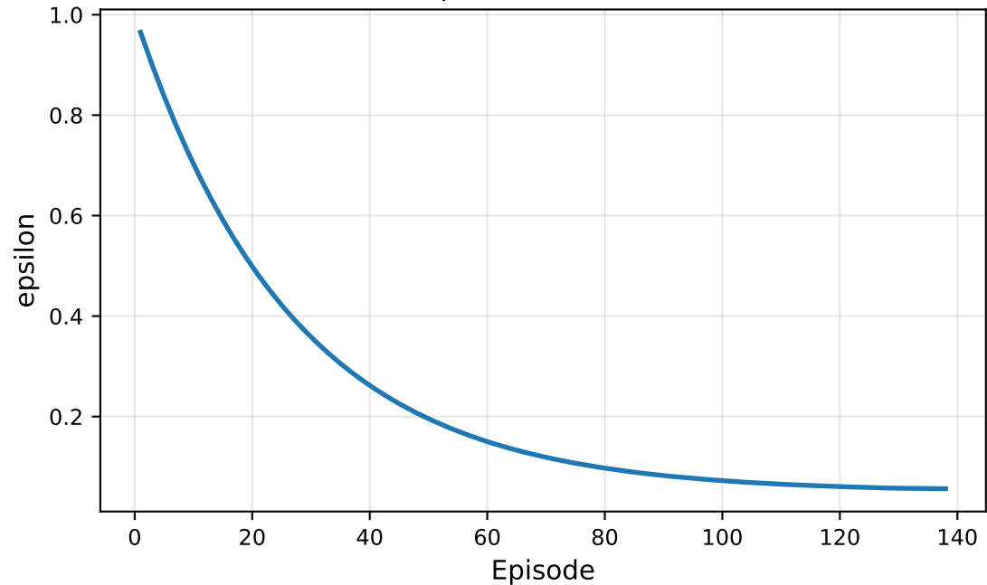
Epsilon schedule
