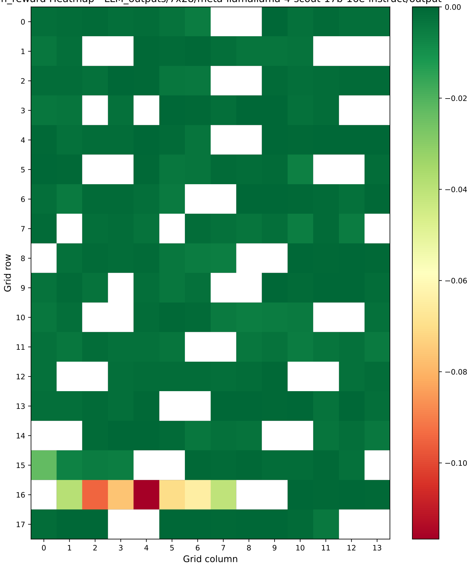
mean_reward Heatmap - LLM_outputs/7x28/meta-llamallama-4-scout-17b-16e-instruct/output
