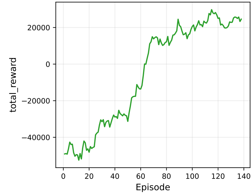
Training reward
