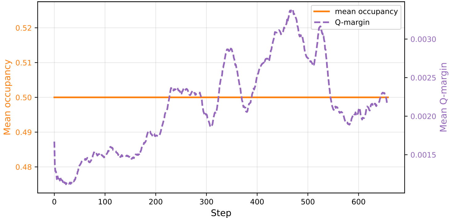
Occupancy and Confidence Margin - LLM_outputs/7x28/meta-llamallama-4-scout-17b-16e-instruct/output
