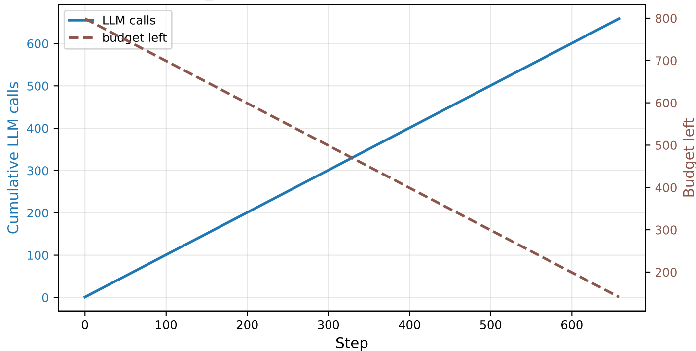
LLM Calls and Budget - LLM_outputs/7x28/meta-llamallama-4-scout-17b-16e-instruct/output
