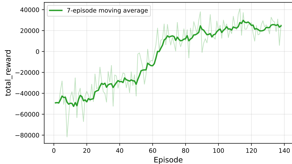
Episode reward
