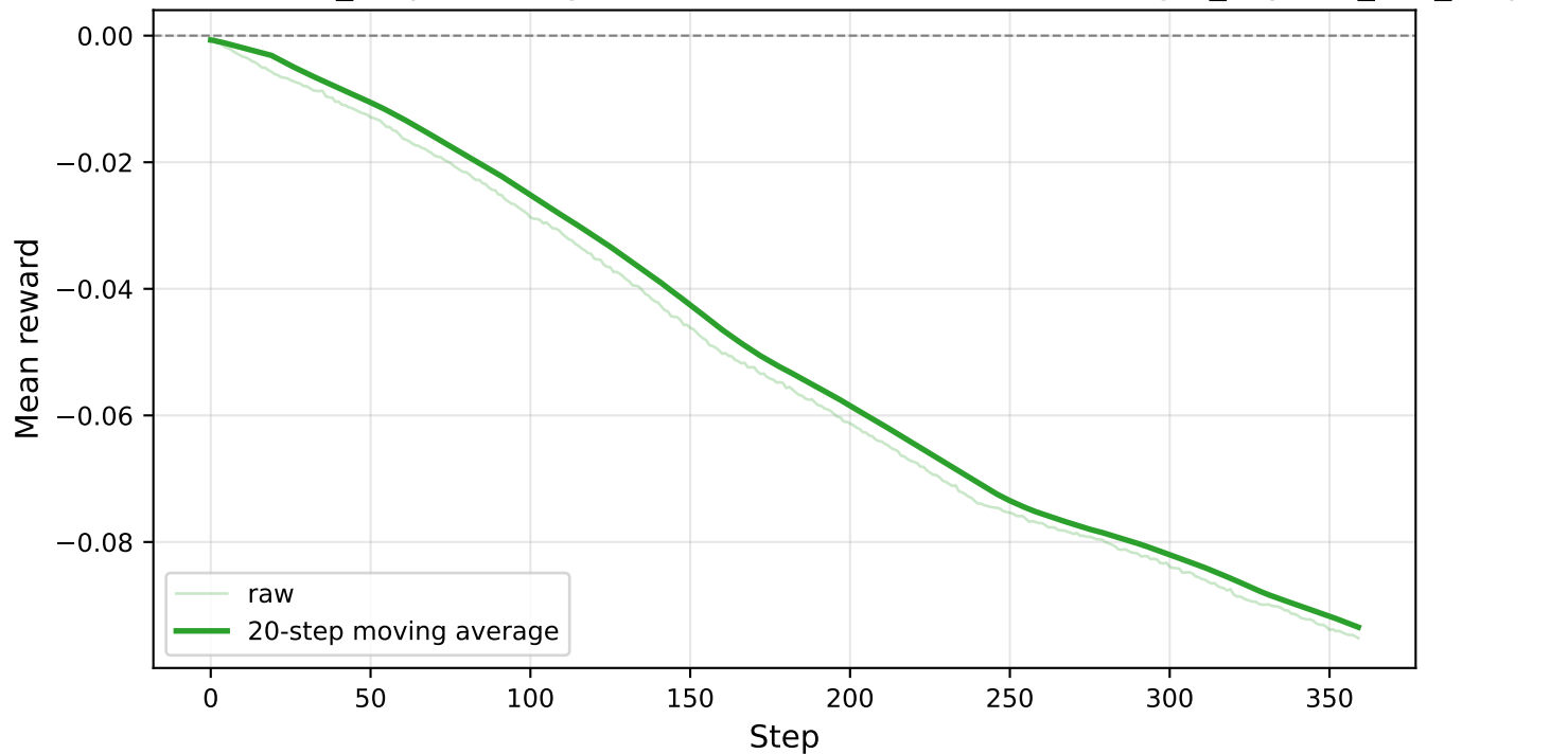
Mean Reward - LLM_outputs/Hangzhou/llama-3.3-70b-versatile/safegat_cityflow_live_output
