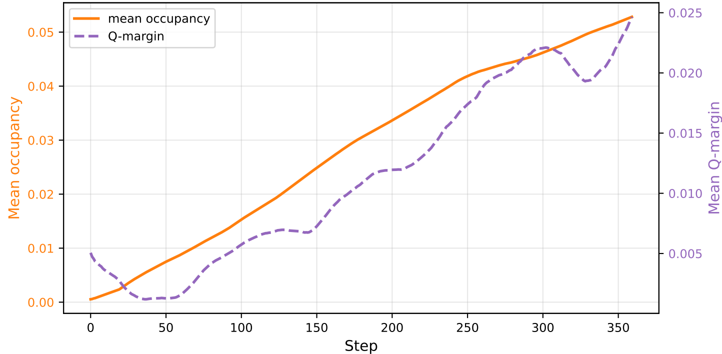
Occupancy and Confidence Margin - LLM_outputs/Hangzhou/llama-3.3-70b-versatile/safegat_cityflow_live_output
