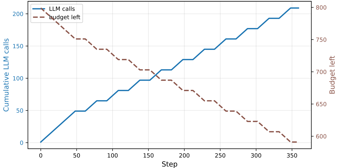
LLM Calls and Budget - LLM_outputs/Hangzhou/llama-3.3-70b-versatile/safegat_cityflow_live_output
