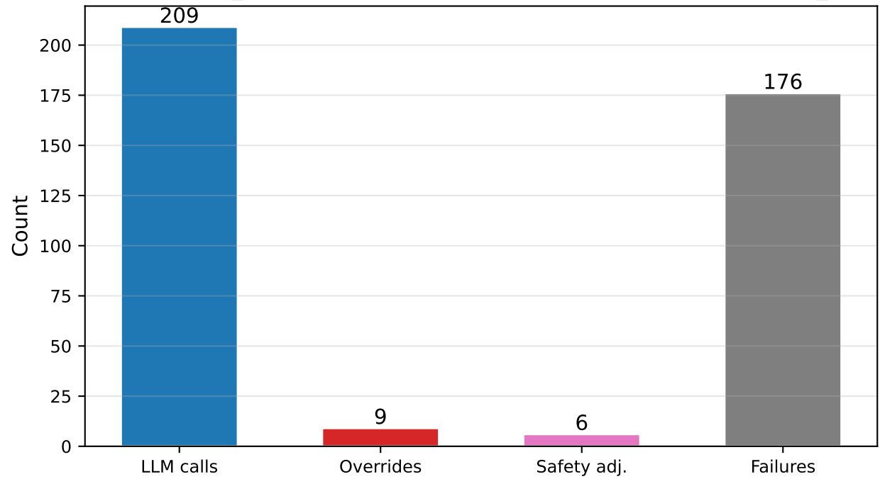
Intervention Summary - LLM_outputs/Hangzhou/llama-3.3-70b-versatile/safegat_cityflow_live_output
