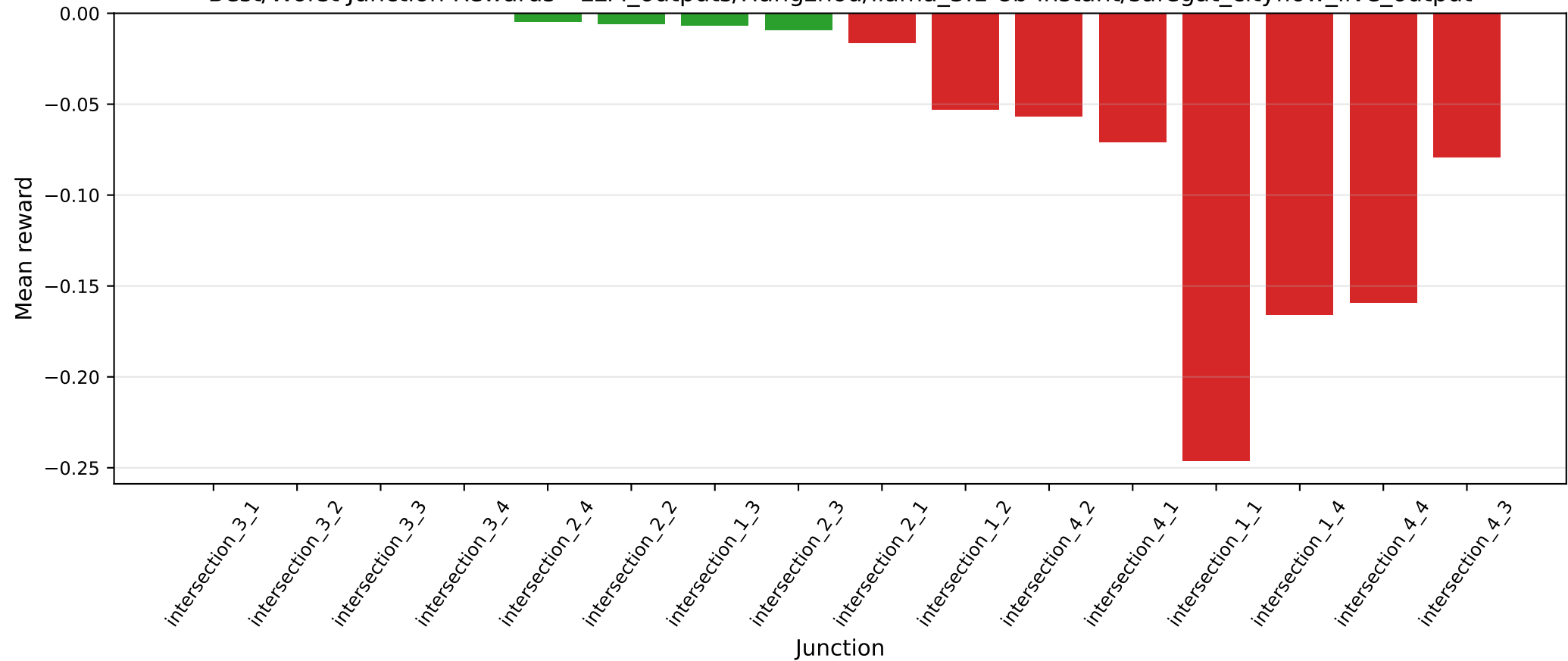
Best/Worst Junction Rewards - LLM_outputs/Hangzhou/llama_3.1-8b-instant/safegat_cityflow_live_output
