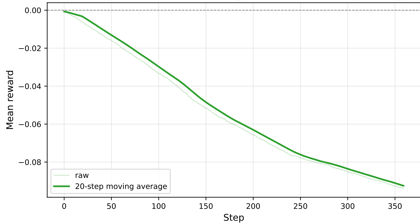
Mean Reward - LLM_outputs/Hangzhou/llama_3.1-8b-instant/safegat_cityflow_live_output
