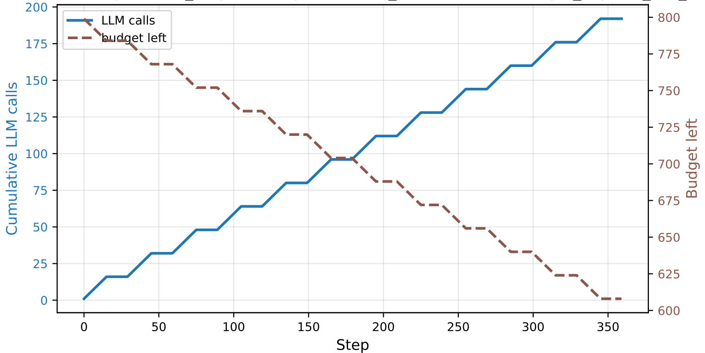
LLM Calls and Budget - LLM_outputs/Hangzhou/llama_3.1-8b-instant/safegat_cityflow_live_output
