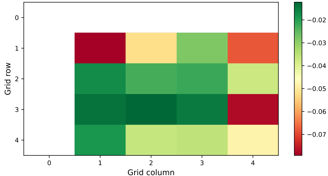
mean_reward Heatmap - LLM_outputs/Hangzhou/meta-llamallama-4-scout-17b-16e-instruct/safegat_cityflow_live_output
