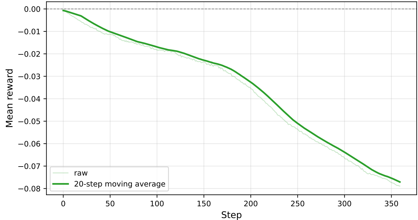
Mean Reward - LLM_outputs/Hangzhou/meta-llamallama-4-scout-17b-16e-instruct/safegat_cityflow_live_output
