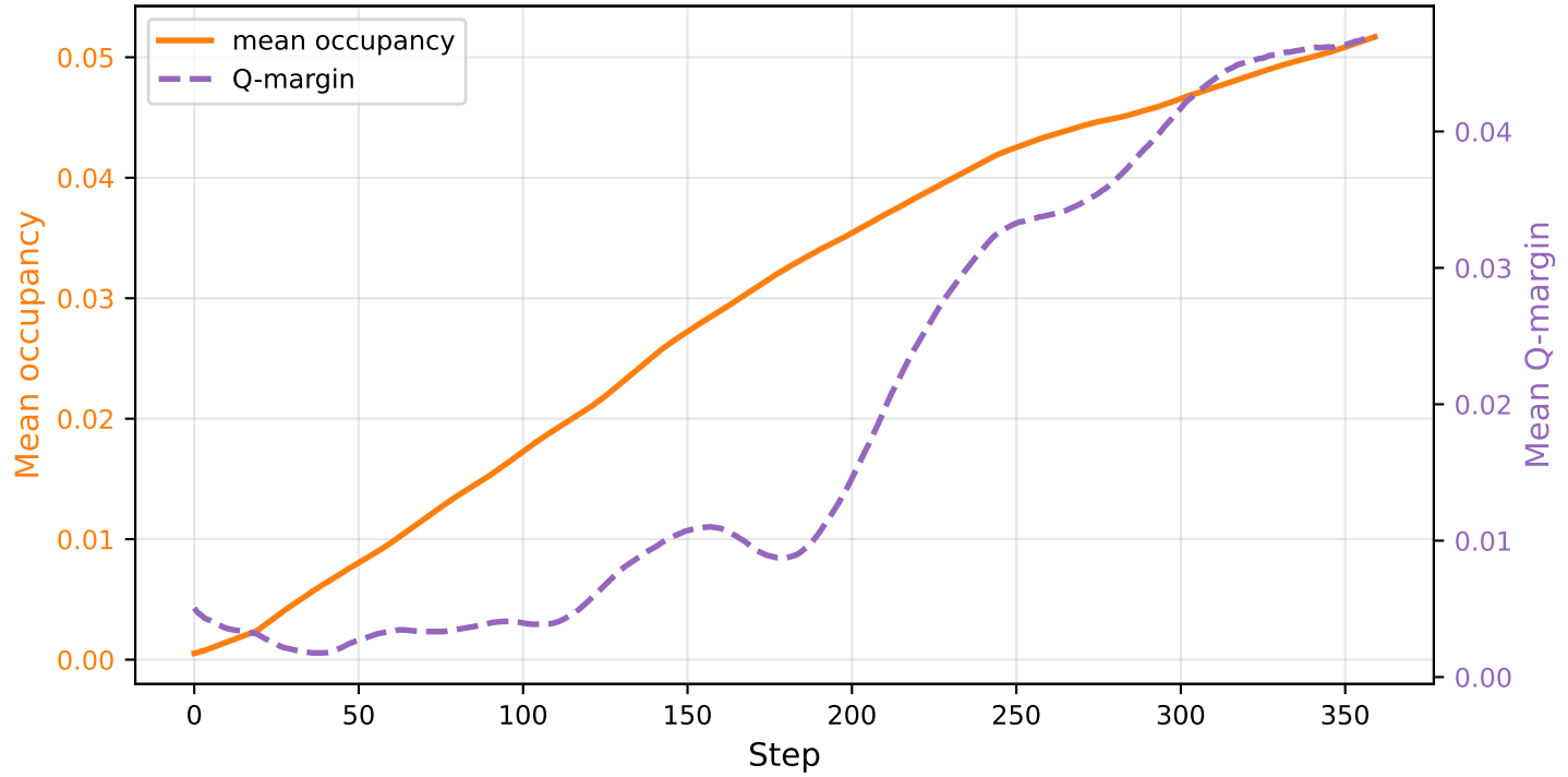
Occupancy and Confidence Margin - LLM_outputs/Hangzhou/openaigpt-oss-120b/safegat_cityflow_live_output
