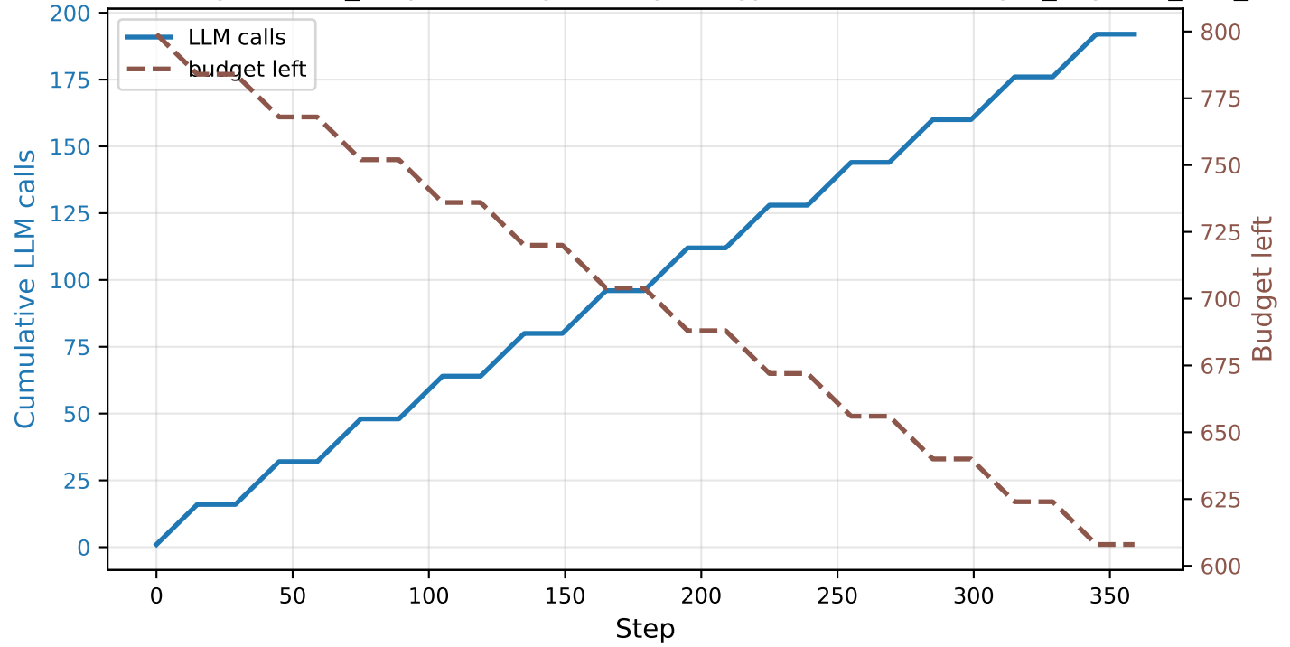
LLM Calls and Budget - LLM_outputs/Hangzhou/openaigpt-oss-120b/safegat_cityflow_live_output
