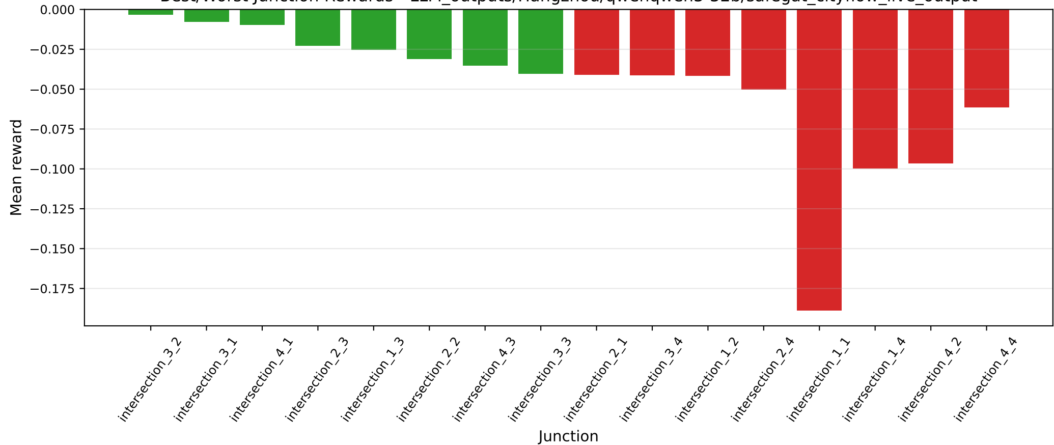
Best/Worst Junction Rewards - LLM_outputs/Hangzhou/qwenqwen3-32b/safegat_cityflow_live_output
