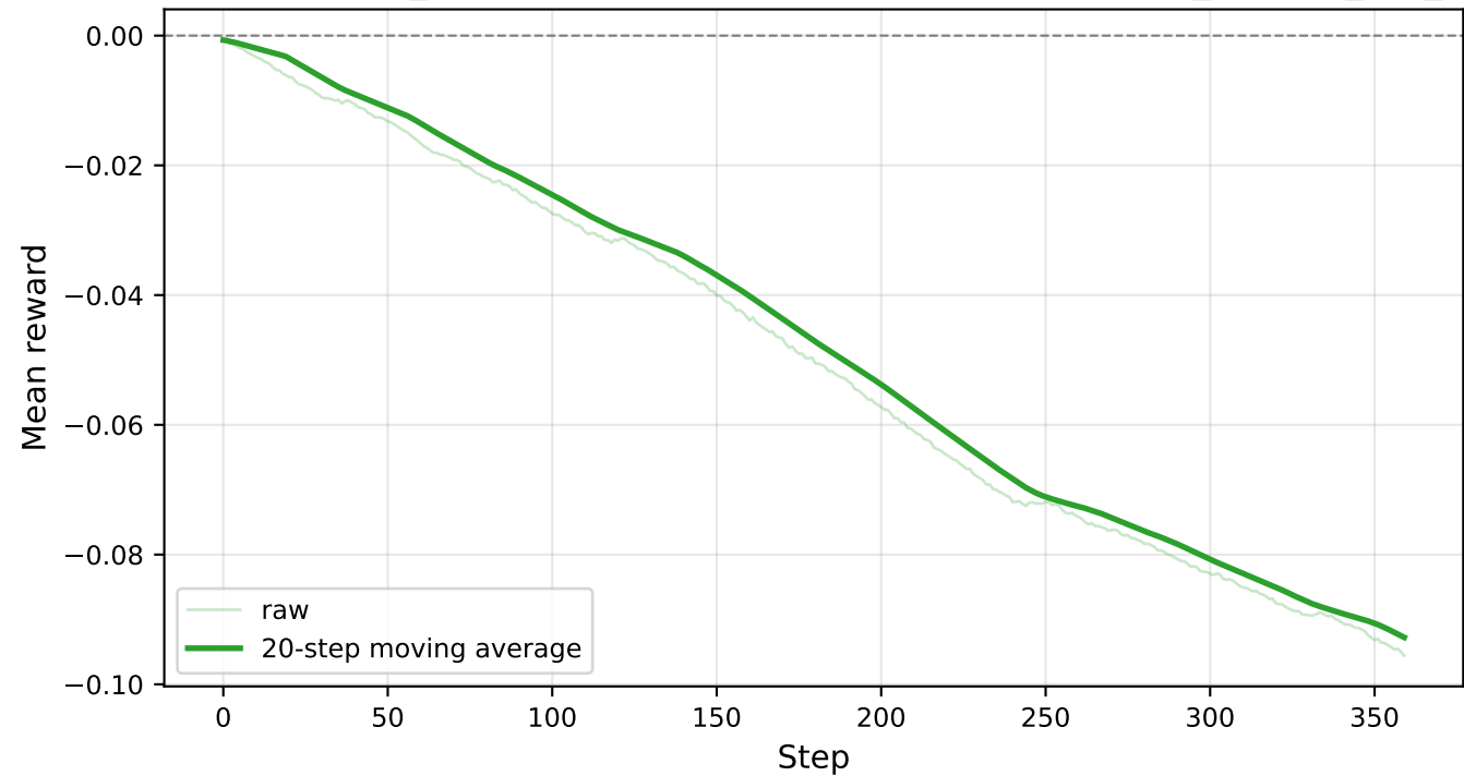
Mean Reward - LLM_outputs/Hangzhou/qwenqwen3-32b/safegat_cityflow_live_output
