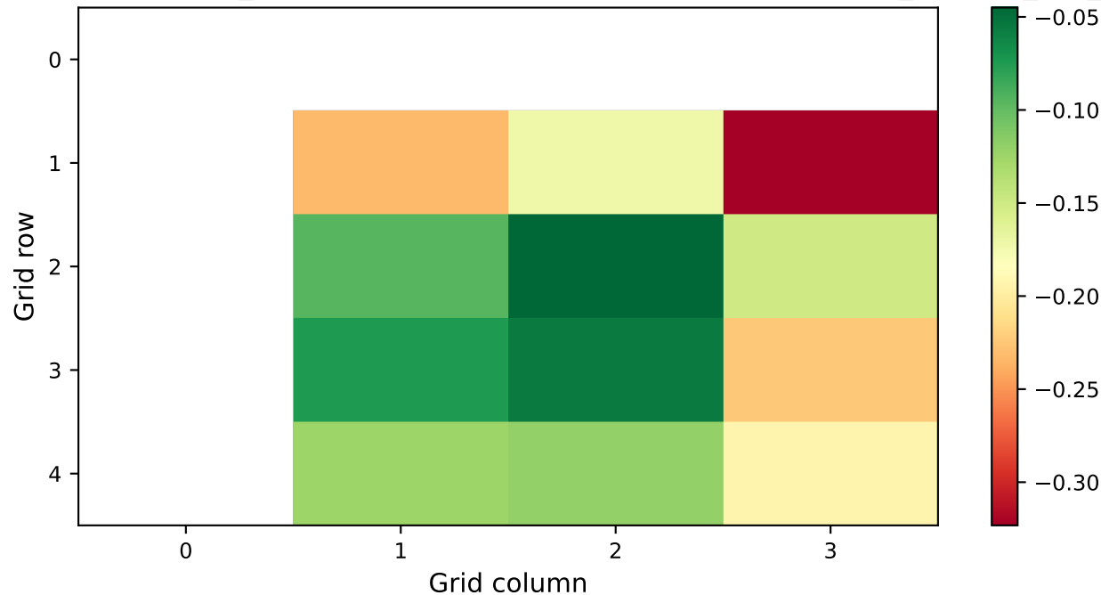
mean_reward Heatmap - LLM_outputs/Jinan/llama-3.3-70b-versatile/safegat_cityflow_live_output
