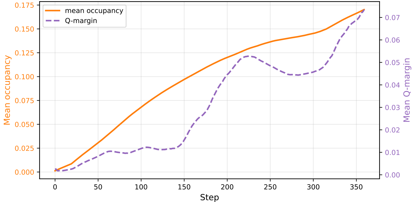
Occupancy and Confidence Margin - LLM_outputs/Jinan/llama-3.3-70b-versatile/safegat_cityflow_live_output
