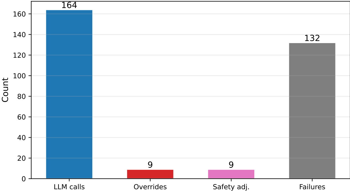
Intervention Summary - LLM_outputs/jinan/llama-3.3-70b-versatile/safegat_cityflow_live_output
