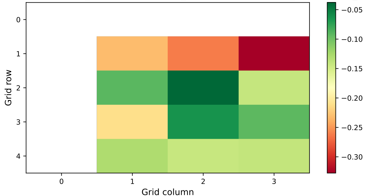
mean_reward Heatmap - LLM_outputs/jinan/llama_3.1-8b-instant/safegat_cityflow_live_output
