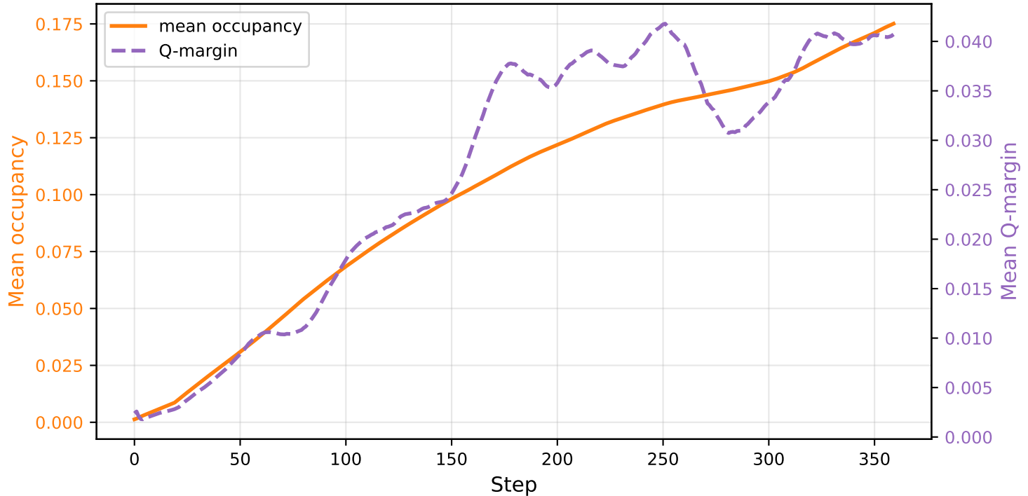
Occupancy and Confidence Margin - LLM_outputs/jinan/llama_3.1-8b-instant/safegat_cityflow_live_output
