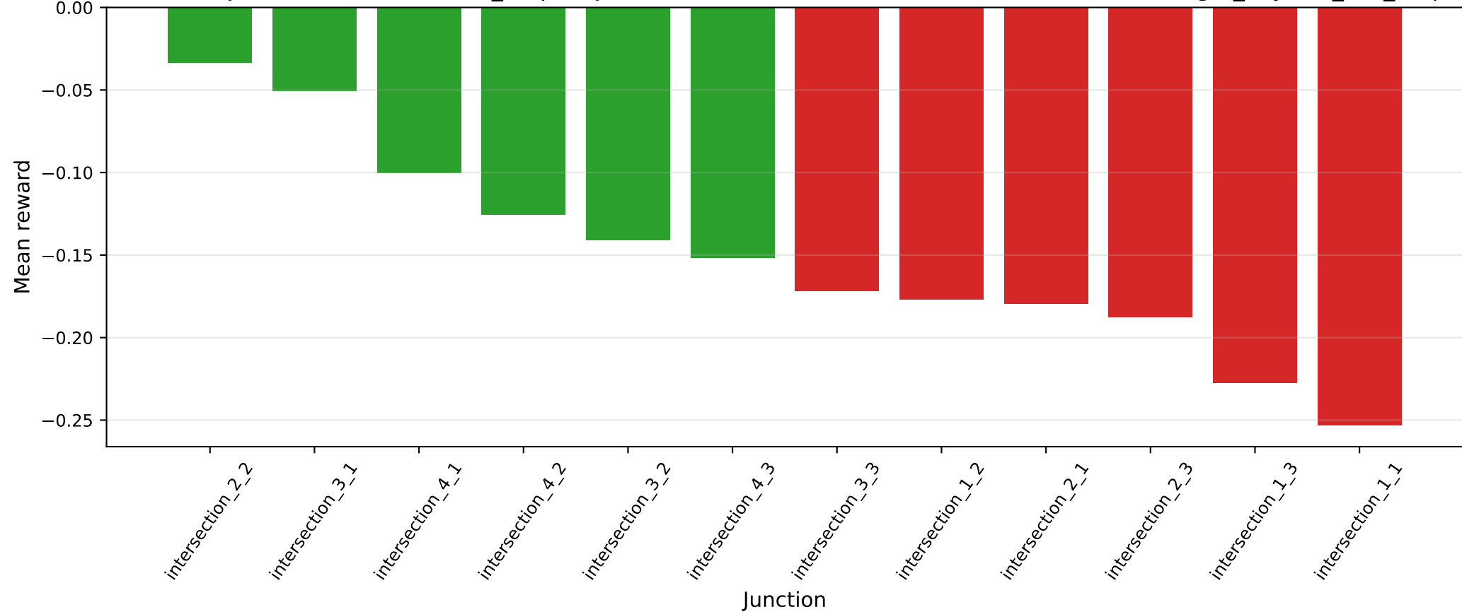
Best/Worst Junction Rewards - LLM_outputs/jinan/meta-llamallama-4-scout-17b-16e-instruct/safegat_cityflow_live_output
