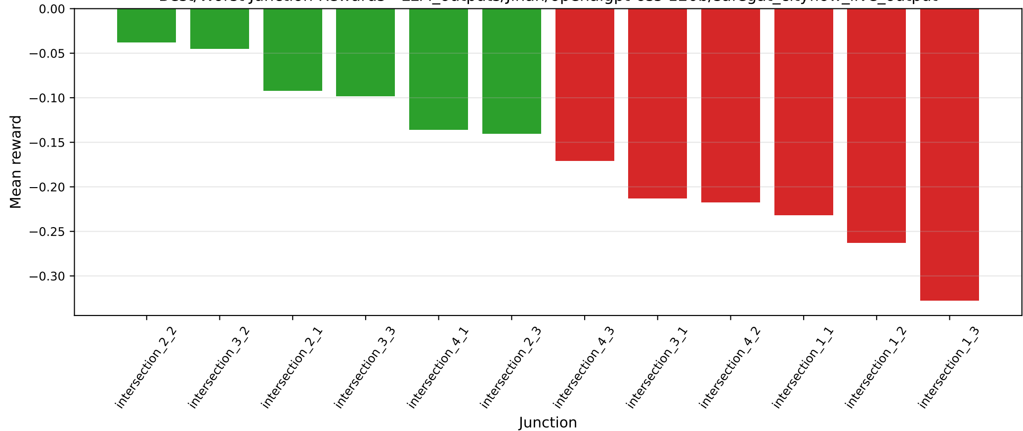
Best/Worst Junction Rewards - LLM_outputs/jinan/openaigpt-oss-120b/safegat_cityflow_live_output
